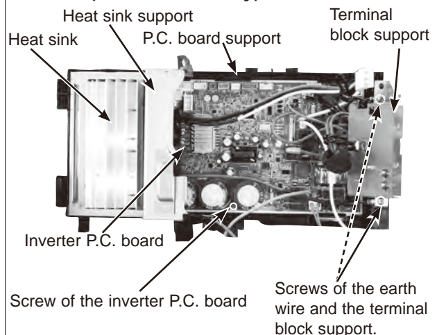
Photo 5 (Inverter assembly)
