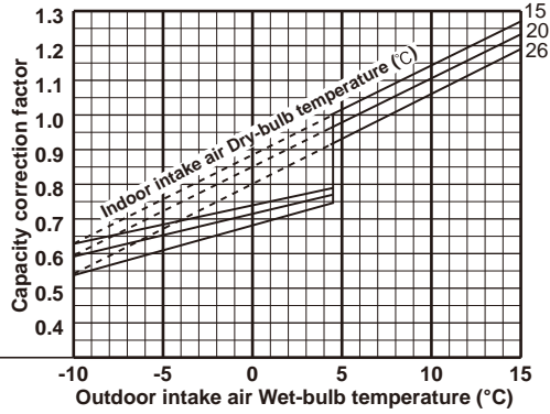
Heating capacity (at Rated frequency)
