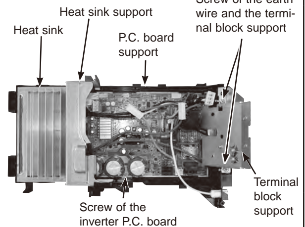
Photo 4 (Inverter assembly)
