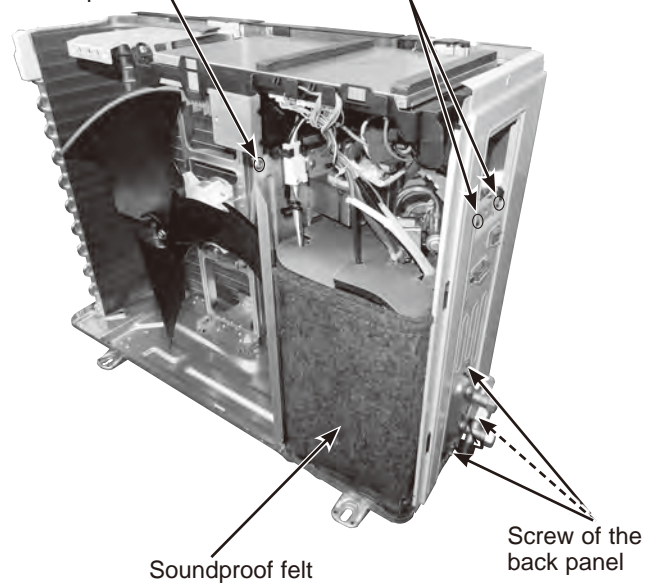
Photo 5 (Inverter assembly)
